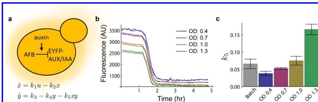
Figure 4. (a) Top: In the presence of auxin, AFB degrades the fusion protein EYFP-AUX/IAA. Bottom: A model from previous work 6 of the network shown. State x represents auxin bound to AFB with input u being the auxin concentration, parameter k_1 the association rate of auxin and AFB, and k_2 the natural degradation rate of AFB. State y represents the concentration of EYFP-AUX/IAA where k_3 is the production rate, k_4 is the natural degradation rate, and k_5 is the degradation rate in the presence of auxin bound to AFB. (b) YKL73 characterized in a turbidostat at four different ODs. At t = 1.25 h auxin was added to the culture chamber and media source to reach a concentration of 10 \mu\text{M} , and the response was measured by sampling effluent and reading mean fluorescence in a flow cytometer at a period of roughly 6 min. The cytometry data was gated to only include singlet (nonbudding) yeast in a healthy size range. An untreated time course is available as Supporting Information Figure S9 and shows no significant change in fluorescence. (c) Model parameter k_5 was fit to the data collected in part b (See Havens et al. 6 Supplemental Data for detailed methods) and compared to previous work (gray). 6
