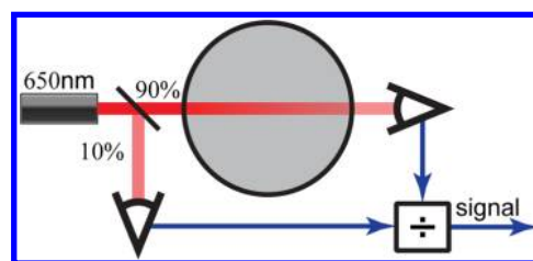
Figure 2. In each chamber, a laser diode emits a 650 nm beam that is then split two ways. Approximately 10% of the light is sent to a photosensor used to measure noise while the remaining 90% is used to measure light transmitted through the cell culture. The ratio of these two signals is a linear function of the transmitted light, which is then normalized to a blank measurement and log transformed to obtain the optical density.
